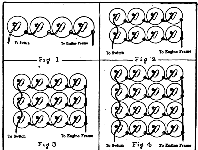
Showing Batteries in Series and in Multiple-Series Relation.
